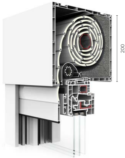
ROLLER SHUTTER BOX 200 mm
