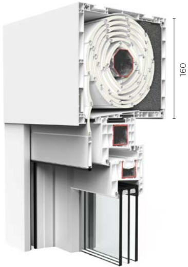
ROLLER SHUTTER BOX 160 mm
