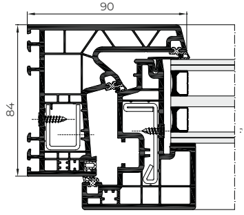
A 84 Hidden Sash
